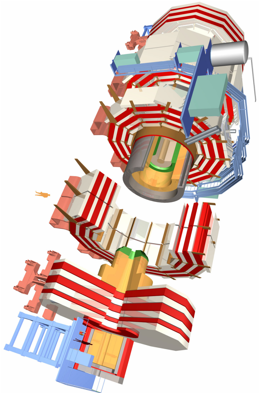
Figure 3.1: A scale schematic of the CMS detector with portions cut-away, movable rings detached to show detail
