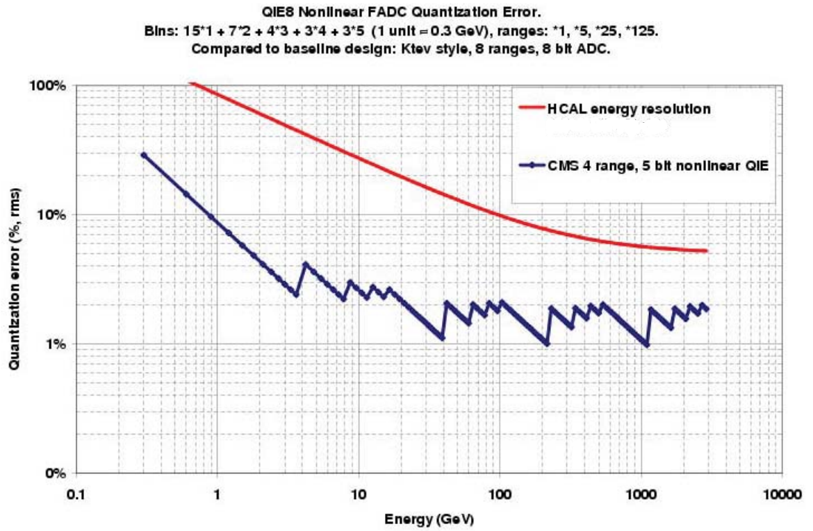
Figure 3.9: Quantization effects of the multi-linear scale of the HB analog-to-digital converters (need better original image, and a time-slice PLOT)
