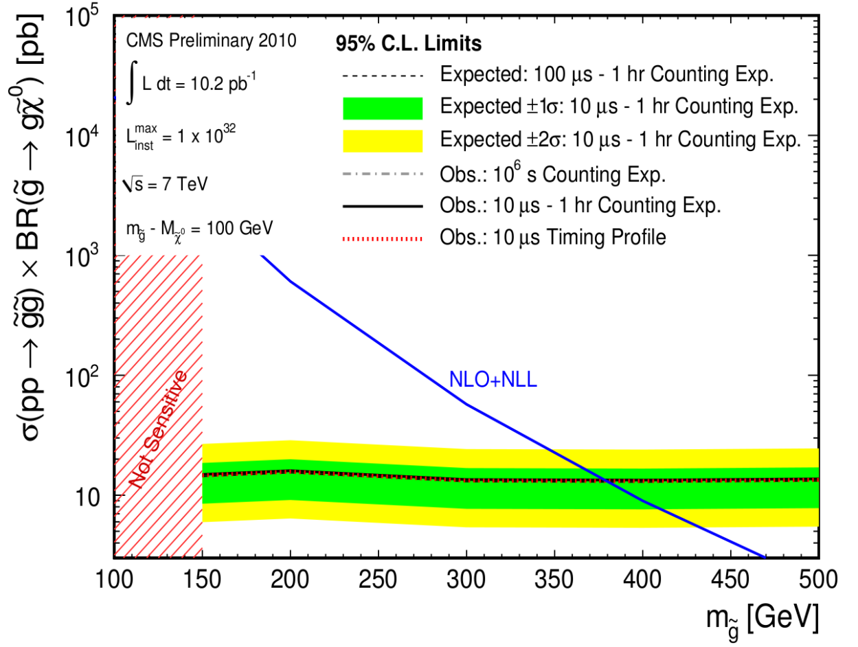
Figure 8.2: Expected and observed 95% C.L. limits on gluino pair production cross-section as a function of gluino mass
