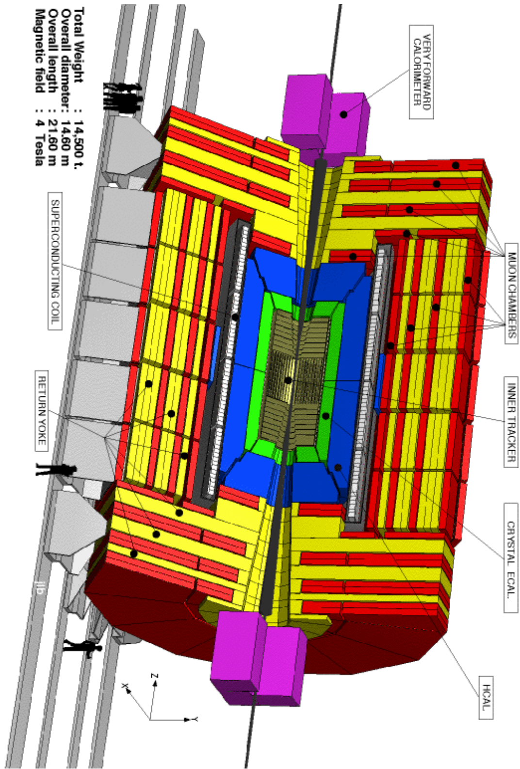
Figure 3.2: A cut-away schematic of the CMS detector, from the CMS Technical Proposal (CITE)
