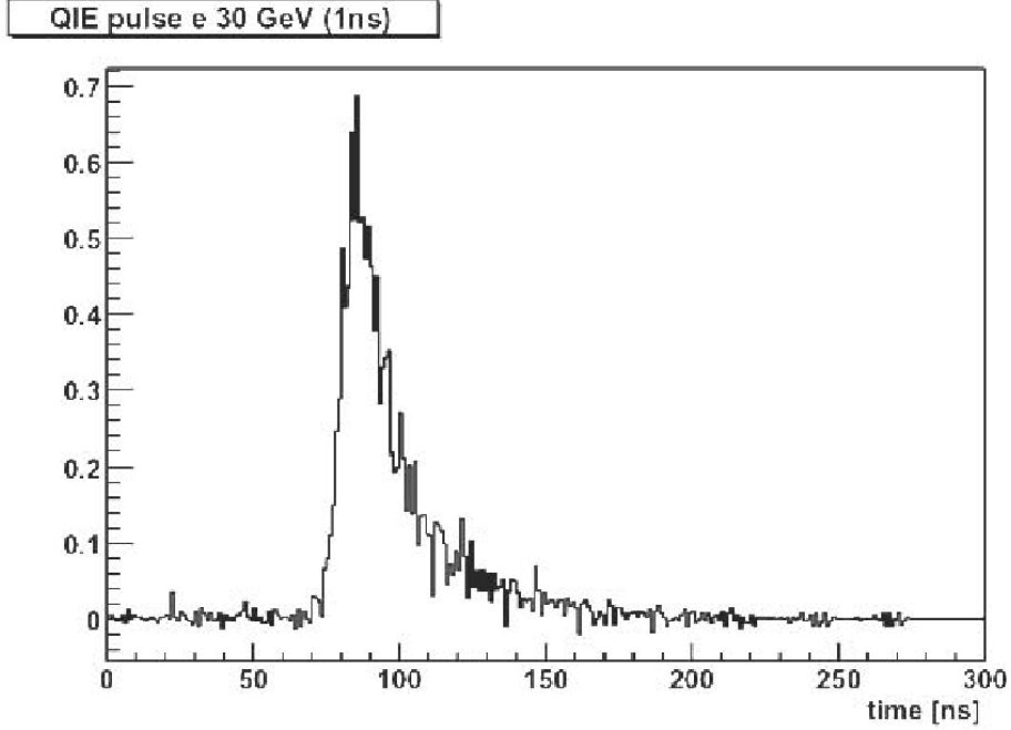
Figure 3.10: A measured pulse of scintillator light characteristic of HB, HE, and HO, taken at a QIE ASIC by a 1 ns sampling-rate oscilloscope (CITE)
