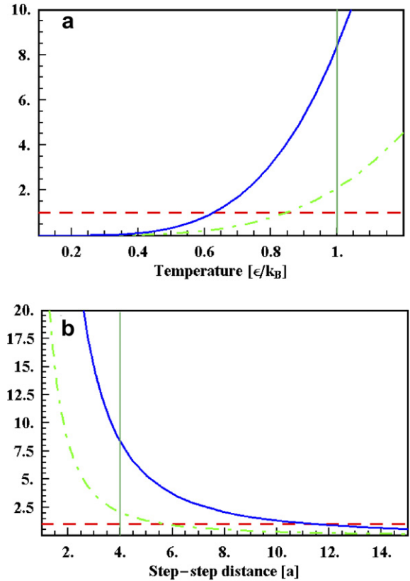
Fig. 2. Magnitude of the three coefficients in Eq. (8) as a function of (a) temperature T[\varepsilon/k_B] ( d=4 ) and (b) step–step distance d[a] ( T=1 ). The fourth-order derivative term, second-order derivative term, and the non-linear KPZ term are given as a dashed, dash-dot and solid line, respectively. The thermodynamic parameters, step free energy \beta , step stiffness \tilde{\beta} and step–step interaction coefficient g , were calculated with the TSK model. The thin vertical line is T=1 and d=4 in (a) and (b), respectively.
