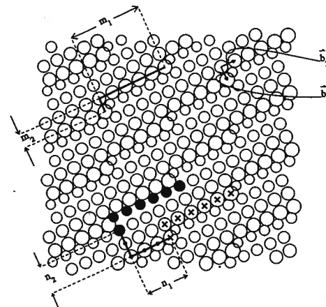
Fig. 1. Nomenclature for surfaces vicinal to (100), in this example (1632). Here m_1 = 5 , m_2 = 1 , n_1 = 3 , n_2 = 2 .
