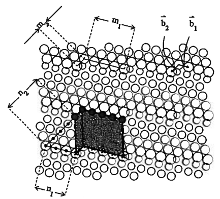
Fig. 2. Nomenclature for surfaces vicinal to (111), in this example (14109). Here m_1 = 4 , m_2 = 1 , n_1 = 3 , n_2 = 4 . The bold lines outline the shaded (111) microfacet of a (14109) unit cell, in this example containing 19 unit cells, as discussed in the appendix.
