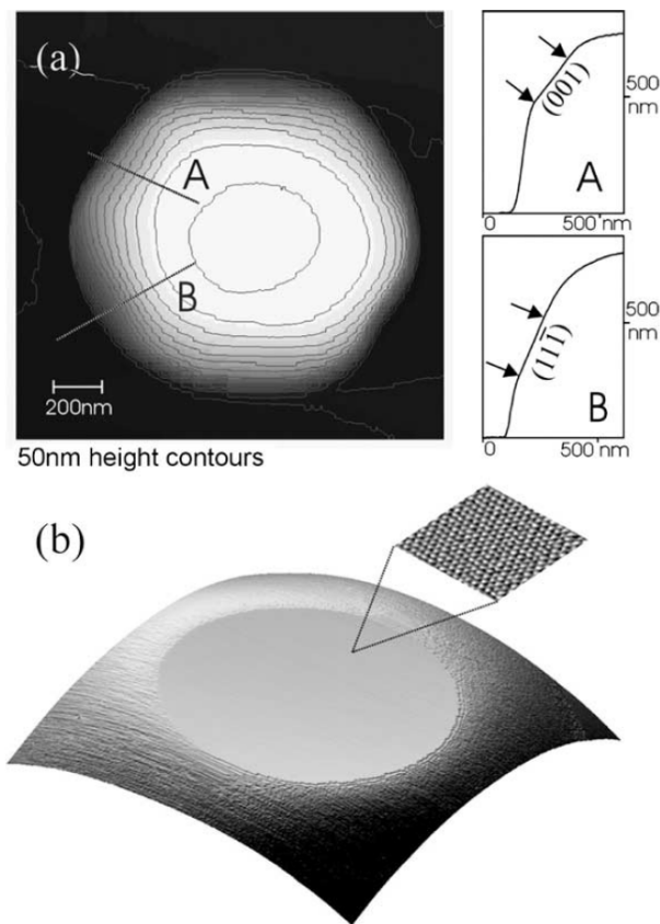
FIG. 18: (a) Micron-size lead crystal (supported on Ru) imaged with a variable-temperature STM at T = 95^\circ\text{C} . Annealing at T = 95^\circ\text{C} for 20 hours allowed it to obtain its stable, regular shape. Lines marked A and B indicate location of profiles. Profile A crosses a (0 0 1)-side facet, while profile B a (1 1 1)-side facet. (b) 770 nm \times 770 nm section of the top part of a Pb-crystal. The insert shows a 5.3 nm \times 5.3 nm area of the top facet, confirming its (1 1 1)-orientation. Both the main image and the insert were obtained at T = 110^\circ\text{C} . From Thürmer et al. [2003].
