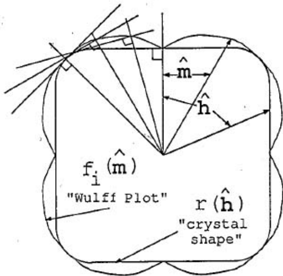
FIG. 3: Schematic of the Wulff construction. The interfacial free energy per unit area f_i \hat{\mathbf{m}} is plotted in polar form (the “Wulff plot” or “ \gamma -plot”). One draws a radius vector in each direction \hat{\mathbf{m}} and constructs a perpendicular plane where this vector hits the Wulff plot. The interior envelope of the family of “Wulff planes” thus formed, expressed algebraically in Eq. (4), is the crystal shape, up to an arbitrary overall scale factor which may be chosen as unity.” From Wortis [1988]
