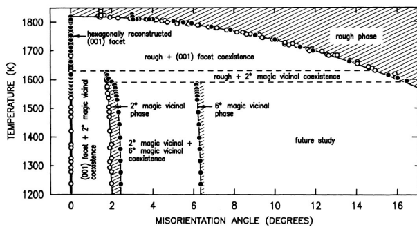
FIG. 24: Orientational phase diagram of vicinal Pt (001) misoriented toward the [110] direction. Single-phase regions are hatched, and two-phase coexistence regions are unhatched. Solid lines are boundaries between two phases. Dashed lines mark triple points. Open circles show misorientation angles measured for a sample miscut by 1.4^\circ towards the [110] direction, while solid circles show tilt angles measured for a sample miscut by 3.0^\circ . From Yoon et al. [1994].
