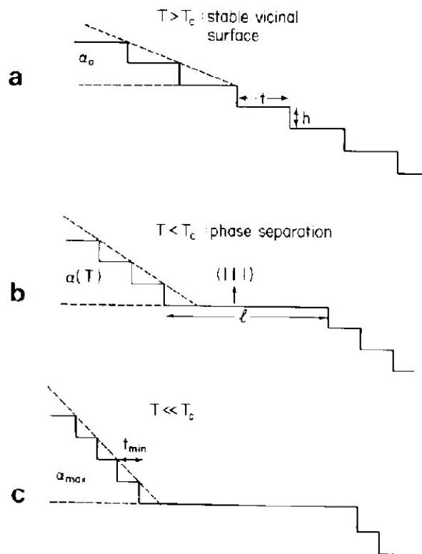
FIG. 23: Microscopic view of what happens to a misoriented surface in Fig. 22 as temperature decreases. (a) At high temperature, the Si(111) vicinal surface is a single, uniform phase. Initial terrace widths t are typically a few nm., as determined by the net angle of miscut \alpha_0 (i.e., \theta_0 ), and the step-height h , which is one interplanar spacing ( \sim 0.31 nm). (b) Below the (7 \times 7) reconstruction temperature ( \sim 850^\circ\text{C} ) the steps cluster to form a new surface of misorientation angle \alpha(T) (i.e., \theta ). A facet of (111) orientation with (7 \times 7) reconstruction forms simultaneously. The width of the (111) facet, l , is larger than the experimentally resolvable width of 500 \text{ \AA} . (c) Well below the transition, the step separation reaches a minimum distance, t_{\min} \sim 1 nm. No further narrowing occurs, perhaps because surface diffusion is too slow T \leq 600^\circ\text{C} . From Williams and Bartelt [1989].
