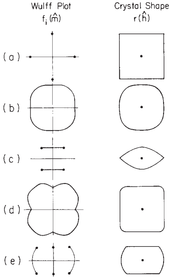
FIG. 6: Some possible Wulff plots and corresponding equilibrium crystal shapes. Faceted and curved surfaces may appear, joined at sharp or smooth edges in a variety of combinations. From Rottman and Wortis [1984a]; the ECS are also in Herring [1953]
