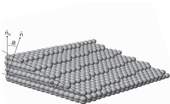
FIG. 1: Portion of a (3\sqrt{2}, 16) surface, vicinal to an fcc (001), to illustrate a misoriented, vicinal surface. The vicinal-surface and terrace normals are \hat{n} = (3, -2, 16)/\sqrt{269} and \hat{n}_0 = (0, 0, 1) , respectively. The polar angle \theta (with respect to the (001) direction), denoted \phi in the original figure (consistent with most of the literature on vicinal surfaces), is \arccos(16/\sqrt{269}) , while azimuthal angle \varphi (denoted \theta in most of the literature on vicinal surfaces), indicating how much \hat{n} is rotated around \hat{n}_0 away from the vertical border on which \theta_0 is marked, is clearly \arctan(1/5) ; \tan \theta_0 = \tan \theta \cos \varphi . Since h is a_1/\sqrt{2} , where a_1 is the nearest-neighbor spacing, the mean distance \ell (in a terrace plane) between steps is a_1/(\sqrt{2} \tan \theta) = 8\sqrt{2/13}a_1 = 3.138a_1 . While the average distance from one step to the next along a principal, (110) direction looks like 3.5a_1 , it is in fact a_1/(\sqrt{2} \tan \theta_0) = 3.2a_1 . The “projected area” of this surface segment, used to compute the surface free energy f_p , is the size of a (001) layer: 20a_1 \times 17a_1 = 340a_1^2 ; the width is 20a_1 . In “Maryland notation” [see text] z is in the \hat{n}_0 direction, while the normal to the vicinal, \hat{n} , lies in the x-z plane and y runs along the mean direction of the edges of the steps. In most discussions, \varphi = 0 , so that this direction would be that of the upper and lower edges of the depicted surface. Adapted from Nelson et al. [1993]
