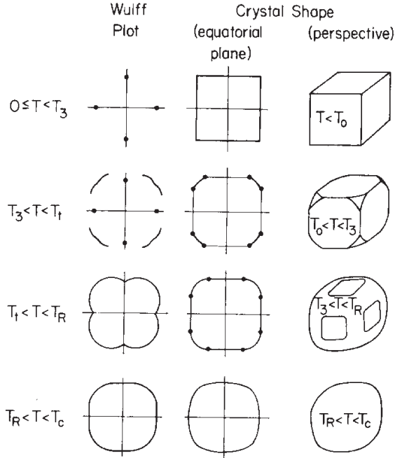
FIG. 15: Representative Wulff plots and ECS's for the crystal with weak NNN repulsions whose phase diagram is shown in Fig.14. Curved surfaces appear first at the cube corners. Junctions between facets and curved surfaces may be either first- or second-order (sharp or smooth), depending on orientation and temperature. From Rottman and Wortis [1984a,b]
