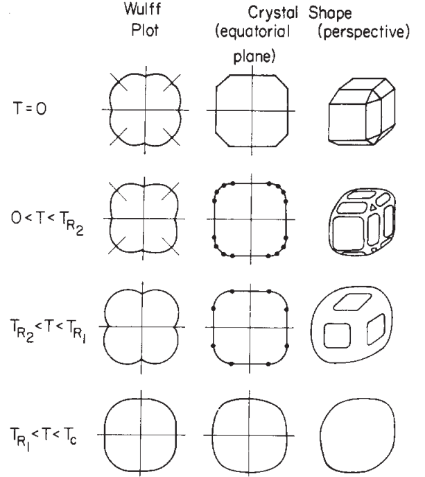
FIG. 13: Representative Wulff plots and ECS’s for the crystal with weak NNN attractions whose phase diagram is shown in Fig.12. At low enough temperature there are (100), (110) and (111) facets. For weak attraction the (110) and (111) facets roughen away below the (100) roughening temperature. For \epsilon_2 = 0 , T_{R2} = 0 , so that the configurations in the second row do not occur; in the first row, the octagon becomes a square and the perspective shape is a cube. Facets are separated at T > 0 by curved surfaces, and all transitions are second order. Spherical symmetry obtains as T approaches melting at T_c . From Rottman and Wortis [1984]
