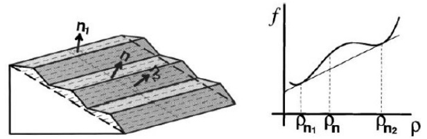
FIG. 7: Illustration of how orientational phase separation occurs when a “hill-and-valley” structure has a lower total surface free energy per area than a flat surface as in Eq. (14). The sketch of the free energy vs. \rho \equiv \tan \theta shows that this situation reflects a region with negative convexity which is accordingly not stable. The dashed line is the tie bar of a Maxwell or double-tangent construction. The misorientations are the coexisting slat-like planes, with orientations \mathbf{n}_1 and \mathbf{n}_2 , in the hill-and-valley structure. From Jeong and Williams [1999]
