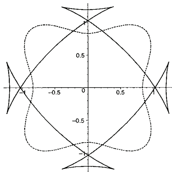
FIG. 10: The solid curve is the \xi plot, while the dashed curve is the 1/\gamma -plot for f_i(\hat{\mathbf{m}}) \equiv \gamma \propto 1 + 0.2 \cos 4\theta . For this case (but not for small values of a ) the 1/\gamma -plot is not convex, and the \xi plot forms “ears.” These ears are then removed, so that the equilibrium shape is given by the interior envelope of the \xi plot, in this case having four corners. From Wheeler [1999]
