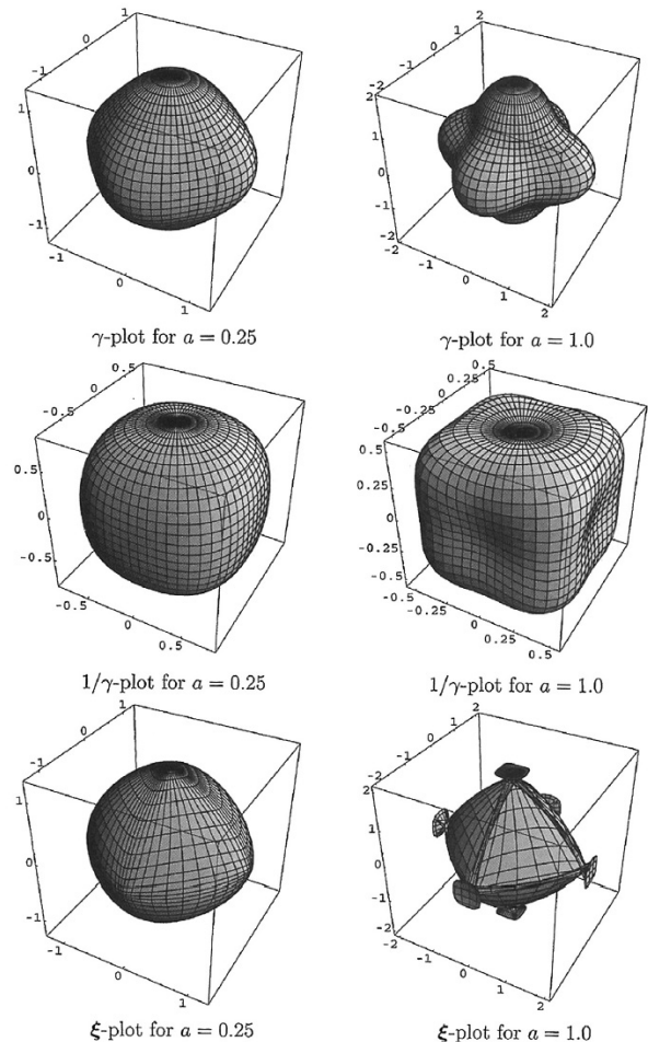
FIG. 2: \gamma -plots (plots of f_i(\hat{\mathbf{m}}) ), 1/\gamma -plots and \xi -plots for Eq. (3) for positive values of a . For a = 1/4 , all orientations appear on the ECS. For a = 1.0 , the 1/\gamma -plot has concave regions, and the \xi -plot has ears and flaps that must be truncated to give the ECS, essentially an octahedron with curved faces. From Sekerka [2004], which shows in a subsequent figure that the \gamma - and 1/\gamma -plots for a = -0.2 and -0.5 resemble the 1/\gamma - and \gamma -plots, respectively, for a = 1/4 and 1.
