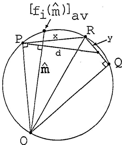
FIG. 8: ECS analogue of the Maxwell double-tangent construction. O is the center of the crystal. Points P and Q are on the (stable) Wulff plot but the region between them is unstable; hence, the ECS follows PRQ and has an edge at R . An interface at the intermediate orientation \hat{\mathbf{m}} breaks up into the orientations P and Q with relative proportions x:y ; thus, the average free energy per unit area given by Eq. (15), which in turn shows that f_i(\hat{\mathbf{m}})_{\text{avr}} lies on the circle. From Wortis [1988]
