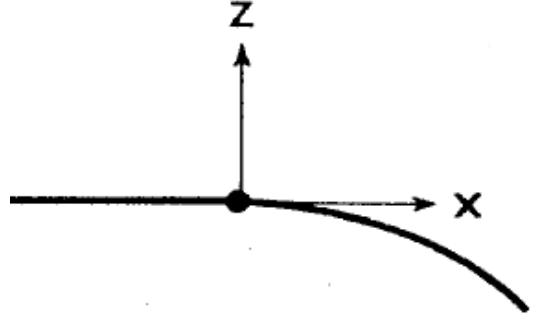
FIG. 17: Critical behavior of the crystal shape near a smooth (second-order) edge, represented by the dot at (x_0, z_0) . The temperature is lower than the roughening temperature of the facet orientation, so that the region to the left of the dot is flat. The curved region to the right of the dot correspond to a broad range of rough orientations. In the thermodynamic limit, the shape of the smoothly curved region near the edge is described by the power law z \sim z_0 - (x - x_0)^\vartheta . Away from the edge there are “corrections to scaling”, i.e. higher-order terms (cf. Eq. (33)). For an actual crystal of any finite size, there is “finite-size rounding” near the edge, which smooths the singular behavior. Adapted from Jayaprakash and Saam [1984]
