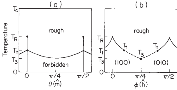
FIG. 14: Interfacial phase diagram with (weak) next-nearest-neighbor (NNN) repulsion rather than attraction as in Fig. 12. The NNN repulsion stabilizes the (100) facets. Curved surfaces first appear at the cube corners and then reach the equatorial plane at T_3 . The transition at the equator remains first order until a higher temperature T_t . The dotted boundaries are first order. A forbidden (coexistence) region appears in the T-\hat{h} phase diagram. From Rottman and Wortis [1984a,b]
