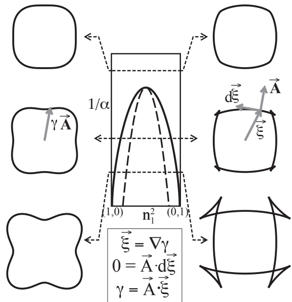
FIG. 9: Graphical constructions for an anisotropic f_i(\hat{\mathbf{m}}) for various values of an anisotropy parameter \alpha , where f_i \propto 1 + \alpha \cos^2 \theta \sin^2 \theta . In the left column f_i(\theta) is plotted from top to bottom for \alpha = 1/2, 1, 2 . Anisotropy increases with positive \alpha , so 1/\alpha corresponds in some sense to a temperature in conventional plots. In the center panel, n_1^2 is \cos^2 \theta . The shape resulting from the gradient construction with the ears removed is the Wulff ECS. From Cahn and Carter [1996]
