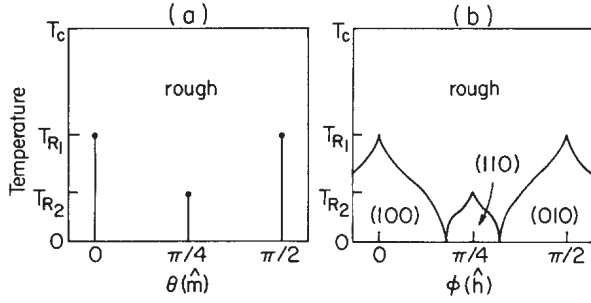
FIG. 12: Interfacial phase diagrams for simple-cubic nearest-neighbor Kossel crystal with nearest-neighbor as well as (weak) next-nearest-neighbor (NNN) attractions. The angular variables \theta and \phi (not to be confused with \varphi , cf. Section 2.2.1) interfacial orientation ( \hat{\mathbf{m}} ) and ECS ( \hat{\mathbf{h}} ), respectively, in an equatorial section of the full 3D phase diagram. a) The T - \theta phase diagram (a) shows the locus of cusps in the Wulff plot along the symmetry directions below the respective roughening temperatures. For no NNN interaction ( \epsilon_2 = 0 ), there are only cusps at vertical lines at 0 and \pi/2 . b) The T - \hat{\mathbf{h}} phase diagram gives the faceted areas of the crystal shape. The NNN attraction leads to additional (111) [not seen in the equatorial plane] and (110) facets at low enough temperature. Thus, for \epsilon_2 = 0 the two bases of the (100) and (010) phases meet and touch each other at (and only at) \phi = \pi/4 (at T = 0 ), with no intervening (110) phase. Each type of facet disappears at its own roughening temperature. Above the phase boundaries enclosing those regions, the crystal surfaces are smoothly curved (i.e., thermodynamically “rough”). This behavior is consistent with the observed phase diagram of hcp ^4\text{He} . From Rottman and Wortis [1984a,b]
