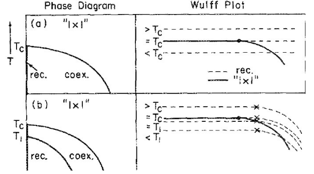
FIG. 22: Wulff plots illustrating the effect of a reconstructive transition on the ECS, and corresponding temperature-[mis]orientation phase diagrams. The solid curves represent the ECS with an unreconstructed [“(1 × 1)”] facet, while the dashed curves give the ECS with a reconstructed facet. As temperature decreases, the free energy of the reconstructed facet, relative to that of the unreconstructed facet, decreases. Below the transition temperature T_c (called T_7 in the text), the two shapes intersect, giving a “net” ECS that is the inner envelope of the two. The phase diagram shows regions where all orientations \tan \theta (or \hat{\mathbf{m}} ) are allowed for the unreconstructed crystal [“(1 × 1)”], regions of phase separation (labeled “coex.”), and regions where the reconstruction (labeled “rec.”) is allowed for ranges of orientation. The relative size of the reconstructed and unreconstructed facets depends on the free energy to create a step on the reconstructed (111) face, compared to its unreconstructed counterpart: (a) the behavior for extremely large energy to create steps on the (7 \times 7) terrace and (b) a smaller such energy. Solid circles mark the sharp edge at the temperature at which the crystal shapes cross. Crosses show the intersection of the facet and the curved part (i.e., the smooth edge) of the crystal shape for the reconstructed phase. From Bartelt et al. [1989].
