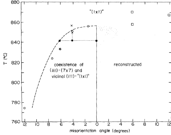
FIG. 21: Summary of experimental results for vicinal Si (111) surface: \circ denotes the temperature at which faceting begins for surfaces misoriented towards the (110) direction, \times the faceting temperatures for surfaces misoriented towards the [1\ 1\ \bar{2}] , and \square the temperatures at which the step structure of surfaces misoriented towards the [\bar{1}\bar{1}2] direction change. The dashed line displays a fit to the [\bar{1}\bar{1}0] data to Eq. (40). The dotted lines show how a 4^\circ sample phase-separates into the states denoted by \bullet as it is further cooled. From Bartelt et al. [1989].
