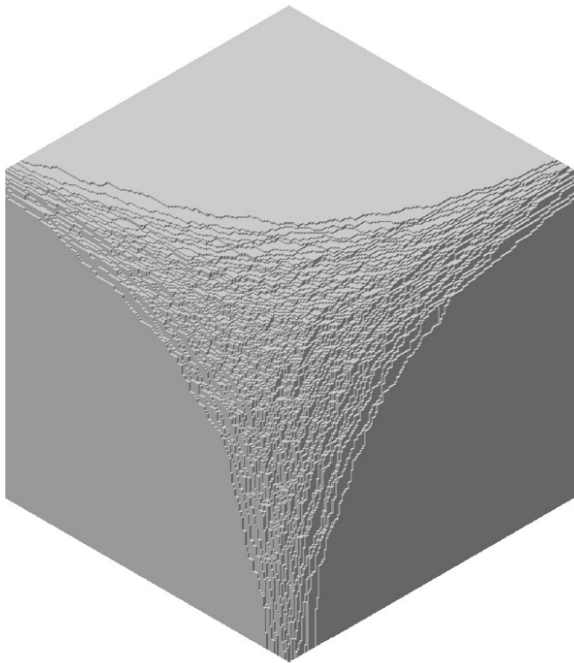
FIG. 19: Simple-cubic crystal corner viewed from the \{111\} direction. From Ferrari et al. [2004].
