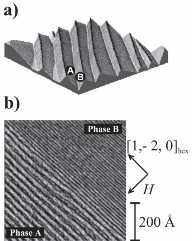
FIG. 11: Morphology of the faceted Au(4,5,5) surface measured at room temperature. (a) 3D plot of a large-scale (scan area: 1.4 \text{ mm} \times 1.4 \text{ mm} ) STM image. Phases A and B form the hill-and-valley morphology. (b) STM image zoomed in on a boundary between the two phases. All steps single-height, i.e. 2.35 \text{ \AA} high. Phase B has smaller terraces, 13 \text{ \AA} wide, while phase A terraces are about 30 \text{ \AA} wide. This particular surface has (2,3,3) orientation. From Rousset [1999]
