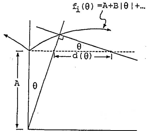
FIG. 5: Wulff plot with a linear cusp at \theta = 0 . If d(\theta) \rightarrow 0 as \theta \rightarrow 0 , then there is no facet corresponding to \theta = 0 , and the \theta = 0 Wulff plane (dotted line) is tangent to the crystal shape at just a single point. Since d(\theta) = B , a cusp in the Wulff plot leads to a facet of the corresponding orientation on the ECS. From Wortis [1988]
