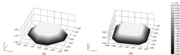
FIG. 25: Perspective views of essentially the ECS (actually the Andreev surface free energy divided by k_B T ) around the (001) facet calculated by the transfer matrix method with the PWFRG algorithm at k_B T/\epsilon_1 = 0.3 . (a) p-RSOS model ( \epsilon_{\text{int}}/\epsilon_1 = -0.5 ). (b) For comparison, the original unsticky RSOS model ( \epsilon_{\text{int}} = 0 ) From Akutsu [2011].
