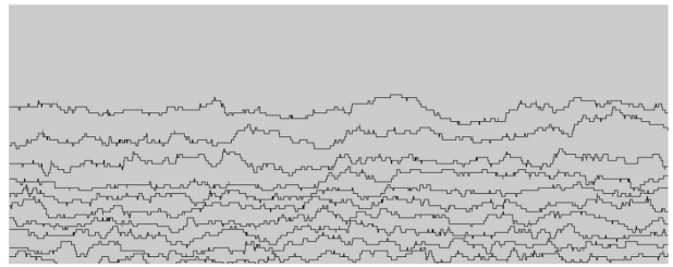
FIG. 20: Magnified detail of the steps near the facet edge, from Ferrari and Spohn [2003]; b) Snapshot of computed configurations of the top steps (those near a facet at the flattened side portion of a cylinder) for a terrace-step-kink (TSK) model with volume constraint. From Ferrari et al. [2004].
