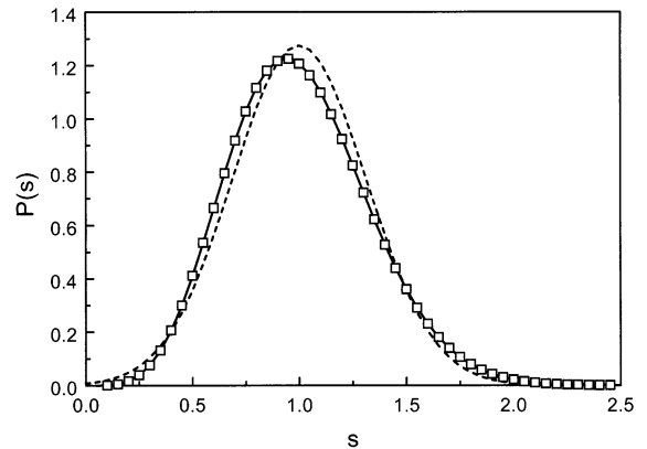
Fig. 2. P(s) versus s \equiv \ell/\langle \ell \rangle for the exactly soluble case \tilde{A}=2 . The small squares, representing an accurate numerical implementation of the exact solution, was generated using a code kindly provided by N.C. Bartelt, which he had developed to produce fig. 5 of Ref. [17]. The standard Gruber–Mullins-like Gaussian approximation is given by the dashed curve. The Wigner distribution for this case, P_4(s) , is the solid curve; it is visually indistinguishable at this scale from the exact solution.
