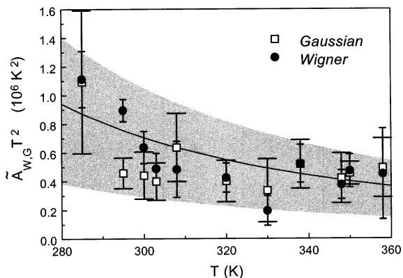
Fig. 6. Temperature dependence of T^2 \tilde{A}_W (solid circles) and T^2 \tilde{A}_G (open squares) for Cu (1 1 13), with error bars distinguished by narrow and wide feet respectively. The solid curve is calculated from Eq. (1), with \tilde{\beta} obtained from Footnote 4 and A set to 7.1 \text{ meV } \text{\AA} , the value determined in Ref. [9]. The gray band blanketing the data corresponds to a range of about \pm 50\% of A .
